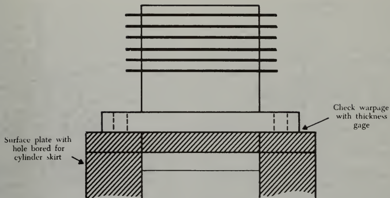
FIGURE 10-3. A method for checking cylinder flange warpage.
